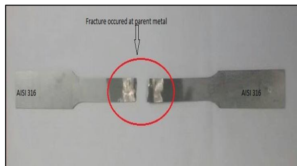
Fig 8: AISI 316-316 Specimen After Tensile Test
