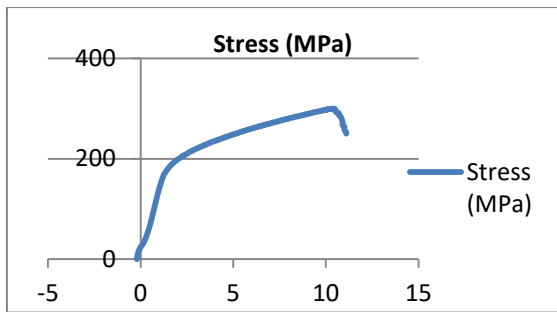
Fig 10: Force vs Displacement Curve Of 304-316 Joint
